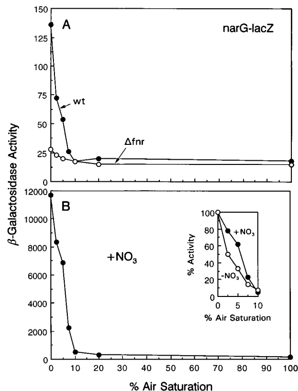
FIG. 2. Effect of oxygen on narG-lacZ expression in the absence (A) and presence (B) of added nitrate. Air saturation is expressed as percent air in the gas stream used for cell growth. The \text{O}_2 content of 100% air-saturated medium is equal to 21% or approximately 230 \mu\text{M} . The wild-type (wt) and fnr ( \Delta fnr ) strains are indicated by the solid and open symbols, respectively. The insert in panel B shows the difference in narG-lacZ expression in cells grown with (●) and without (○) nitrate additions. Data are from the activity levels shown in panels A and B.
