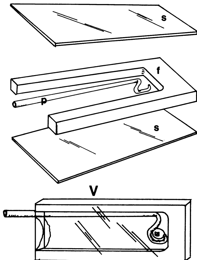
FIG. 2. Construction of microscopic chambers. s, Glass microscope slide; p, bent Pasteur pipette tip; f, plastic frame; V, general view, when assembled and sealed.
