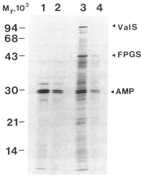
FIG. 3. Expression of plasmid-dependent proteins in maxicells. E. coli DR1984 cells were transformed with plasmid D5 (lanes 3 and 4) or pUC13 (lanes 1 and 2), and extracts were analyzed by electrophoresis on sodium dodecyl sulfate-13% polyacrylamide gels and by autoradiography. The positions of the gene products encoded by the plasmids are indicated by arrowheads at right. The positions of coelectrophoresed standards are indicated by their molecular weights at left.
