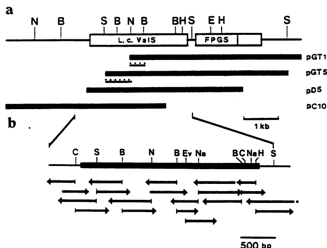
FIG. 1. Cloning, restriction map, and sequencing strategy of the valS gene. (a) The upper section is a restriction map of the segment of L. casei genomic DNA contained in the overlapping clones shown below as solid bars. The large open boxes represent open reading frames, and names are given inside the boxes for those products whose functions are known. The narrow bars with broken lines above them represent DNA fragments of the clones shown above that were used as probes to isolate the clones shown below. (b) The region of L. casei DNA that was sequenced is shown with an expanded restriction map. The solid bar represents the open reading frame of the valS gene. The solid arrows show stretches of sequence determined from single templates. Arrows beginning at vertical bars represent sequences determined from plasmids deleted at the restriction site denoted by the bar. If the vertical bar is not present, the sequence was determined from the end of a subclone (upper section) originating at a Sau3AI site not shown on the map. The arrow at right originating at a solid square represents sequence determined from a specific primer which was previously described (23). Restriction enzyme abbreviations are as follows: N, NcoI ; B, BamHI ; S, SphI ; H, HindIII ; E, EcoRI ; Na, NarI ; Ev, EcoRV ; C, Clai .
