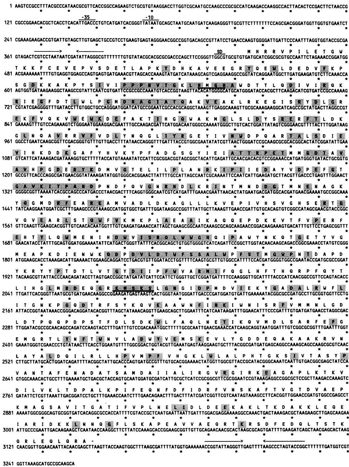
FIG. 2. Nucleotide sequence of the L. casei valS gene and flanking regions. The deduced amino acid sequence of the VRS is shown above the nucleotide sequence. The consensus -10 and -35 putative promoter sequences 5' to the open reading frame are overlined. The deduced Shine-Dalgarno sequence is indicated by overlining. Potential terminator sequences in the 5' and 3' noncoding regions are indicated by converging arrows. The termination codon is indicated with a dash. Amino acid residues that are identical to those in the other three reported valS genes, VRSBS, VRSEC, and VRSSC, are shaded. The consensus HIGH and KMSKS sequence motifs for class I tRNA synthetases are double underlined.
