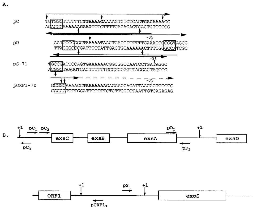
FIG. 5. Summary of the MALA3A2 footprinted regions and the ExsA consensus element. (A) DNase I footprint summary for pC, pD, and pS (54). The pS promoter region was footprinted as the entire PstI-NsiI fragment but is represented as separate promoters in this article. The -35 sites as determined from transcriptional start site mapping (53, 54) are shown. Strong protection is indicated by solid horizontal arrows, and weak protection is indicated by the broken arrow. The ExsA consensus element is in bold print. Nucleotides with enhanced DNase I cleavage (vertical arrows) and GCGG boxes (boxed areas) are shown. (B) Schematic of the trans -regulatory and exoS loci showing the position and orientation of the ExsA consensus elements. Mapped transcriptional start sites are shown as vertical arrows; the positions and orientations of the ExsA consensus element (TXAAAXA) are shown as horizontal arrows.
