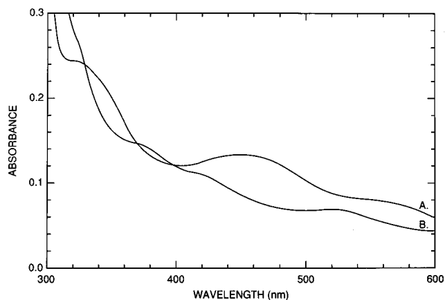
FIG. 3. Absorption spectra of ISP BPH (2.08 mg of protein per ml in a 1-ml total volume). (A) Oxidized; (B) reduced with NADPH in the presence of catalytic amounts (50 \mu g each) of reductase BPH and ferredoxin BPH .
