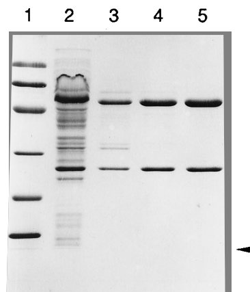
FIG. 2. SDS-PAGE analysis of samples taken during the purification of ISP_{BPH} . Lanes: 1, molecular weight markers; 2, cell extract (15 \mu g of protein); 3, Q-Sepharose column fractions containing ISP_{BPH} (3.0 \mu g of protein); 4, phenyl-Sepharose column fractions containing ISP_{BPH} (3.4 \mu g of protein); 5, hydroxyapatite column fractions containing ISP_{BPH} (3.0 \mu g of protein). The arrowhead denotes the dye front.
