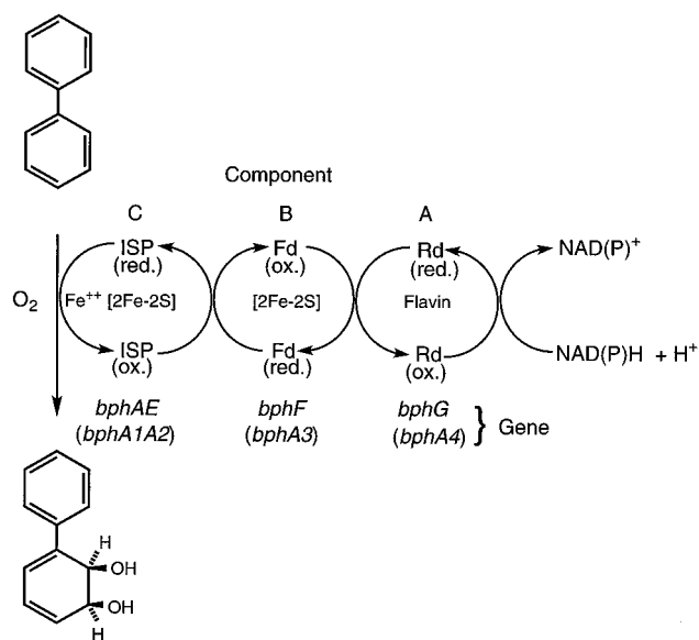
FIG. 5. Proposed arrangement of the protein components of biphenyl 2,3-dioxygenase. Abbreviations: Fd, ferredoxin BPH ; Rd, reductase BPH ; red., reduced; ox., oxidized. A, B, and C are designations given to the three components following resolution by anion-exchange column chromatography (27).
