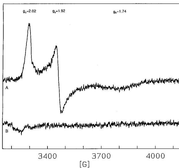
FIG. 4. EPR spectra of ISP BPH (1.2 mg of protein; 7.8 mg/ml). (A) Reduced with sodium dithionite; (B) oxidized.
