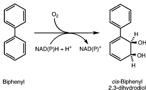
FIG. 1. Reaction catalyzed by biphenyl 2,3-dioxygenase.
