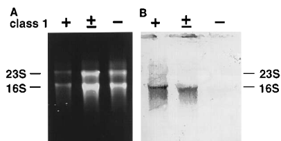
FIG. 3. Northern hybridization analysis of total RNA of class 1 outer membrane protein expression variants of N. meningitidis isolate 2257. (A) Ethidium bromide-stained gel. The 16S and 23S ribosomal RNA species are indicated. (B) Hybridization with the DIG-labeled PCR product of primers P21 and P22. From a duplicate gel, the RNA was transferred to a nylon membrane and porA -specific RNA was detected by hybridization. Strong (+) or moderate (±) expression or the absence of (-) expression of the class 1 protein is indicated.
