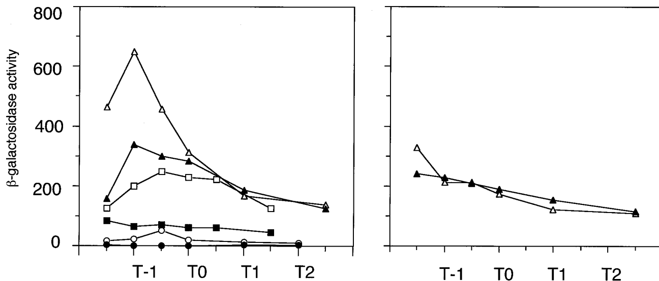
FIG. 5. Effect of nucleotide alteration from a \sigma^D - to a \sigma^A -type -10 sequence. (A) Reduction of the suppressive effect of pLC1 on degR expression; (B) inability of pLC1 to suppress degR expression in a sigD mutant. The scales on the y axes in the two panels are the same. The details of the drawings are described in the legend to Fig. 3. The numbers on the x axis represent the growth time in hours relative to the end of vegetative growth (T0). Growth conditions and measurement of \beta -galactosidase activities were identical to those in the legend to Fig. 1 except that the culture media contained both kanamycin and chloramphenicol (A) or kanamycin, chloramphenicol, and phleomycin (B).
