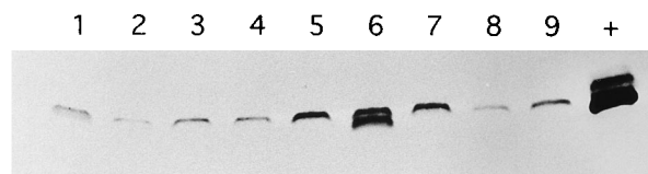
FIG. 7. Western blot of TEM-1 \beta -lactamase and mutants selected for ceftazidime ( 0.5 \mu\text{g ml}^{-1} ) hydrolytic activity. Three mutants from each random library selection were selected for expression studies. Lanes: 1, 177-DNA-179; 2, 177-CWN-179; 3, 177-QWY-179; 4, 174-ENF-176; 5, 174-LLL-176; 6, 174-DDN-176; 7, 171-DQR-173; 8, 171-HKA-173; 9, 171-ERR-173; +, wild type.
