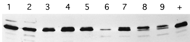
FIG. 6. Western blot of TEM-1 \beta -lactamase and mutants selected for ampicillin ( 1 \text{ mg ml}^{-1} ) hydrolytic activity. Three mutants from each random library selection were selected for expression studies. Lanes: 1, 177-PRD-179; 2, 177-VND-179; 3, 177-EQD-179; 4, 174-PCD-176; 5, 174-AED-176; 6, 174-LLD-176; 7, 171-DAI-173; 8, 171-GAA-173; 9, 171-HAT-173; +, wild type.
