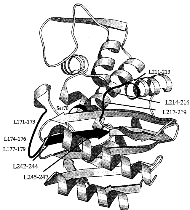
FIG. 2. Ribbon diagram of TEM-1 \beta -lactamase. The locations of the randomized library positions are indicated. The figure was prepared by using MOLSCRIPT (16).
