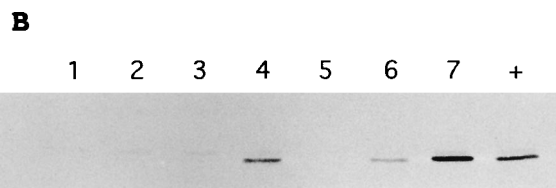
FIG. 8. Expression and resistance characteristics of the mutations which make up the 165-YYG-167 triple mutant. This mutant was isolated previously by selecting for mutants resistant to 15 \mu\text{g} of ceftazidime \text{ml}^{-1} . (A) MICs for 165-YYG-167 triple mutant and its elemental single and double mutants. The MICs of ampicillin (AMP) and ceftazidime (CAZ) are shown on the right. The type of mutant (single, double, or triple) is indicated on the left. (B) Expression of 165-YYG-167 triple mutant and its elemental single and double mutants demonstrated by Western blot analysis. Lanes: 1, 165-YYG-167 triple mutant; 2, 165-WYG-167 double mutant; 3, 165-YEG-167 double mutant; 4, 165-YYP-167 double mutant; 5, 165-WEG-167 single mutant; 6, 165-WYP-167 single mutant; 7, 165-YEP-167 mutant; +, 165-WEP-167 wild-type TEM-1 \beta -lactamase.
