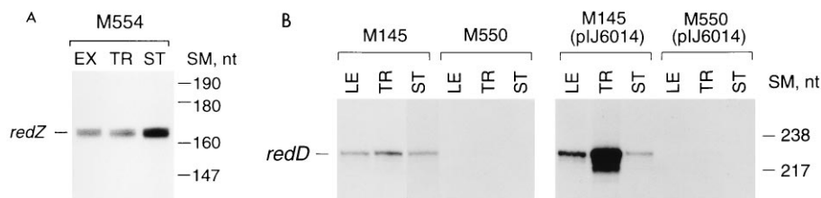
FIG. 5. Analysis of the transcriptional dependence between redZ and redD . (A) Transcription of redZ in the redD mutant M554. RNA was isolated from a liquid (SMM)-grown culture during exponential growth (EX), transition phase (TR), and stationary phase (ST) and used in S1 nuclease protection studies with a uniquely end-labelled probe specific for redZ transcripts that should yield a protected fragment of 166 nucleotides (nt). (B) Transcription of redD in M145, in the redZ mutant M550, and in derivatives of each containing pIJ6014. RNA was isolated from liquid (SMM)-grown cultures during late exponential growth (LE), transition phase (TR), and stationary phase (ST) and used in S1 nuclease protection studies with a uniquely end-labelled probe specific for redD transcripts that should yield a protected fragment of 229 nucleotides. SM, end-labelled Hpa II-digested pBR322 size markers.
