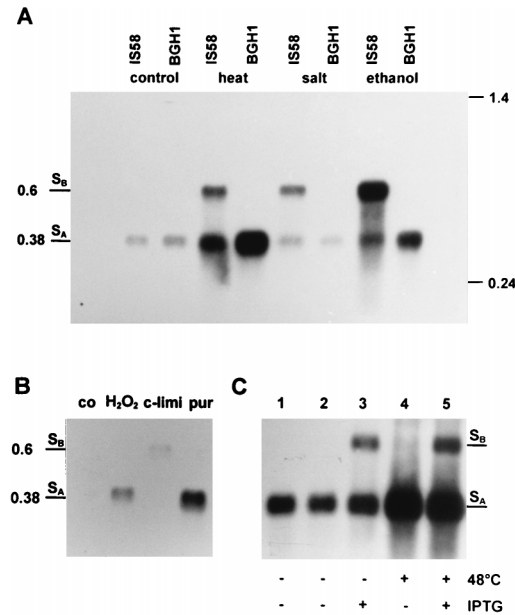
FIG. 4. Northern blot analysis. (A) RNA was isolated from B. subtilis IS58 (wild type) and BGH1 ( sigB ) at 37°C (control) and 9 min after a temperature shift to 48°C (heat) or after the addition of 4% NaCl (salt) or 4% ethanol (ethanol). The RNA was separated under denaturing conditions, transferred to a nylon membrane, and hybridized with a digoxigenin-labeled RNA probe specific for trxA . The locations of molecular size standards (in kilobases) and of mRNAs with 5' ends at S_B and S_A are marked. (B) Total RNA was isolated from the wild-type strain, IS58, during exponential growth (co), 9 min after exposure to 0.0002% H_2O_2 ( H_2O_2 ) or 20 \mu g of puromycin (pur/ml) or 30 min after the cells entered the stationary phase as a result of the exhaustion of glucose (c-limi). The samples were processed as described for panel A. (C) RNA was isolated from B. subtilis BSA115 before (lane 1) or 6 min after exposure (+) to 48°C heat stress (lane 4), from bacteria grown in the absence (-) (lane 2) or presence (+) (lane 3) of IPTG, and after a combination of heat shock and the addition of IPTG (lane 5).
