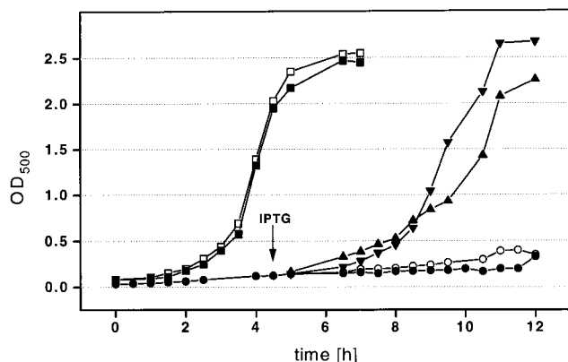
FIG. 6. Effect of variations in the level of TrxA on the growth of B. subtilis . The B. subtilis strain BIG1, in which the expression of trxA is controlled by P_{SPAC} was grown in the presence of 50 \mu M IPTG and diluted 30-fold into fresh prewarmed Luria broth with or without 50 \mu M IPTG. At the time indicated by the arrow different concentrations of IPTG were added to the cultures incubated without IPTG. The wild-type strain, IS58, is included as a control. ■, IS58 control; □, BIG1 with 50 \mu M IPTG added immediately; ●, BIG1 without IPTG; ○, BIG1 with 5 \mu M IPTG; ▲, BIG1 with 10 \mu M IPTG; ▼, BIG1 with 50 \mu M IPTG. OD 500 , optical density at 500 nm.
