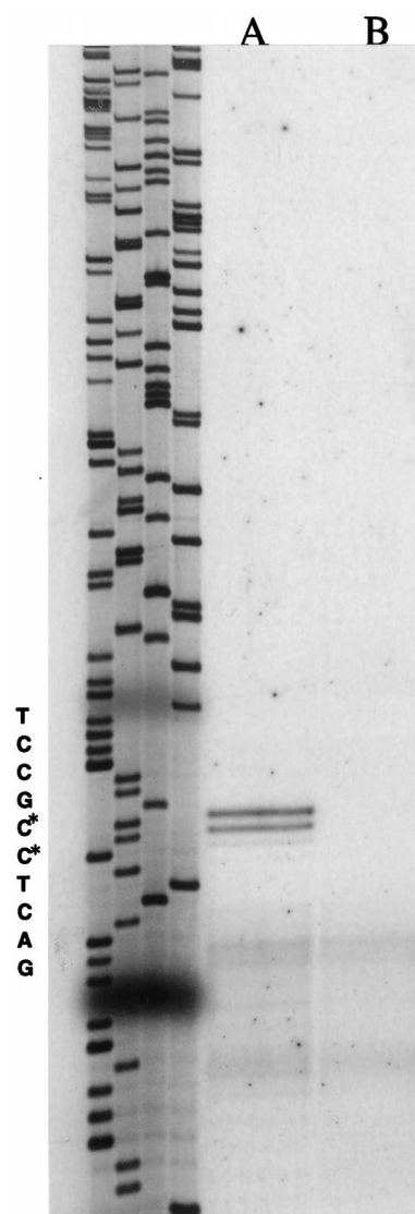
FIG. 3. Reverse transcriptase mapping of the transcriptional start site of the ptb gene in B. subtilis 168 grown in the presence (lane A) or absence (lane B) of 20 mM isoleucine. The positions of the cDNA-extended fragments identified with oligonucleotide O 1 were compared with those obtained by sequencing of an M13 recombinant phage containing the promoter region with the same oligonucleotide used as a primer (lanes at left, TCGA, respectively, from left to right). Transcriptional start sites are indicated by the asterisks.
