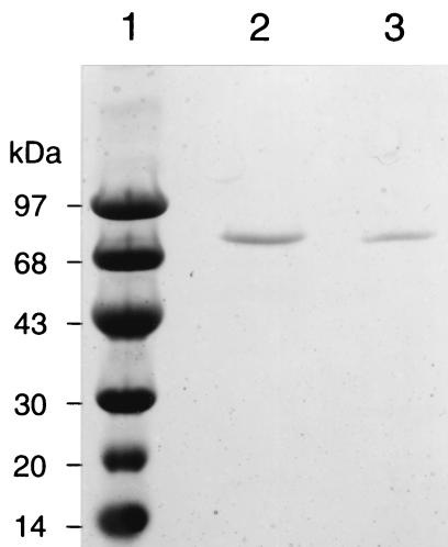
FIG. 4. Electrophoresis of the purified CL190 and E. coli DXP synthase overexpressed in E. coli . Purified DXP synthases of CL190 and E. coli obtained by using a Ni-nitrotriocetic acid agarose column were analyzed by SDS-8 to 25% PAGE. Lanes: 1, molecular mass standard; 2, SDS-treated CL190 enzyme (0.2 \mu\text{g} ); 3, SDS-treated E. coli enzyme (0.1 \mu\text{g} ). Proteins were stained with Coomassie brilliant blue R-250.
