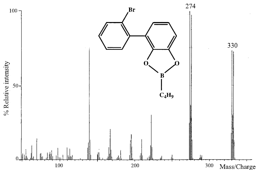
FIG. 3. Mass spectra of n -butylboronate derivatives of dioxxygenation products. Major metabolites of 2,2'-difluoro- (A) and 2,2'-dibromo-biphenyl (B) are shown. The assigned structures are shown as inserts.
