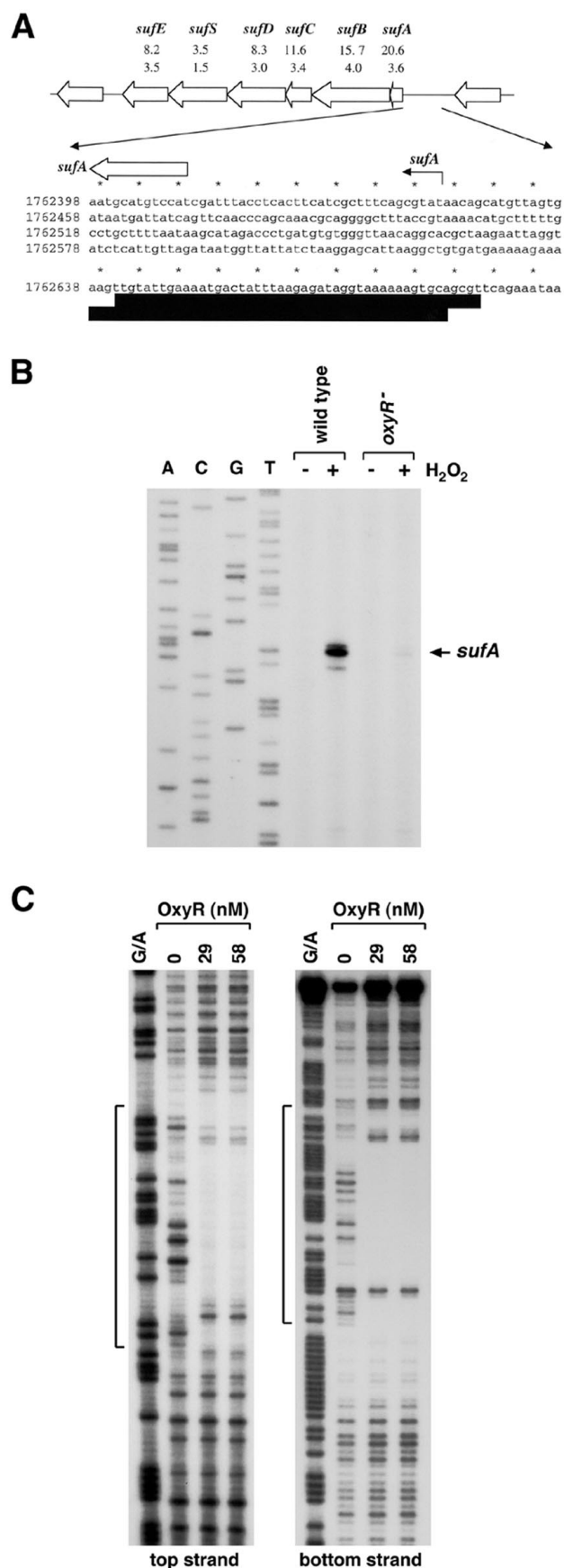
FIG. 2. OxyR-dependent induction of the suf operon. (A) Structure of the suf operon and sequence of the sufA promoter. The induction ratios observed for the wild-type and \Delta oxyR mutant strains in the microarray experiment are given below each gene. The sufA transcription start is marked by the black arrow, and the start of the corresponding ORF is denoted by a white arrow. The DNase I footprints for OxyR binding are indicated by the dark boxes. Our computational search (41) predicted an OxyR binding site of 9.6 bits centered at position 922026. (B) Primer extension assays of sufA expression in wild-type (MC4100) and \Delta oxyR (GSO47) strains grown in LB medium. Exponential-phase cultures were split into two aliquots: one aliquot was left untreated, and the other was treated with 1 mM hydrogen peroxide. The cells were harvested after 10 min, total RNA was isolated, and primer extension assays were carried out with primer 820 specific to sufA . The neighboring sequencing reactions were carried out with the same primer. (C) DNase I footprinting assays of oxidized OxyR binding to the top and bottom strands relative to the sufA promoter. The regions protected by OxyR on both strands are indicated by the brackets. For OxyR binding to the top strand, the 32 P-labeled primer 828 and unlabeled primer 825 were used to PCR amplify a 187-bp fragment. For OxyR binding to the bottom strand, the 378-bp NotI - Bam HI fragment of pGSO133 was labeled with 32 P at the Bam HI site. The samples were run in parallel with Maxam-Gilbert G/A sequencing ladders.
