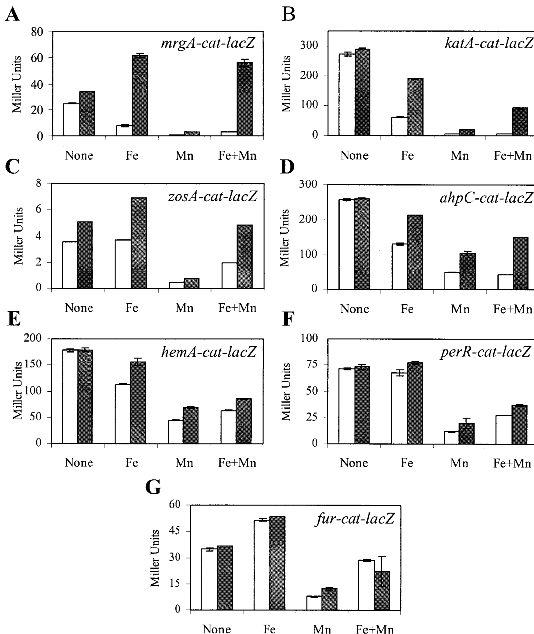
FIG. 6. Induction of PerR regulon genes by H 2 O 2 . Strains containing the indicated reporter fusions were grown in minimal medium with no added Mn(II) or Fe(III) (None) or with 10 μM Fe(III) (Fe), 5 μM Mn(II) (Mn), or both (Fe+Mn) as described in the legend to Fig. 3. At 2 h after resuspension, the cultures were split and 100 μM H 2 O 2 was added to one sample. After growth for another 30 min, cells were harvested for β-Gal assay and induced expression (gray bars) was compared to expression in the absence of H 2 O 2 addition (white bars). Note that the data represented by the white bars are the same as those for the 2.5-h time point in Fig. 3. Experiments were performed twice; error bars represent the standard error of the mean.
