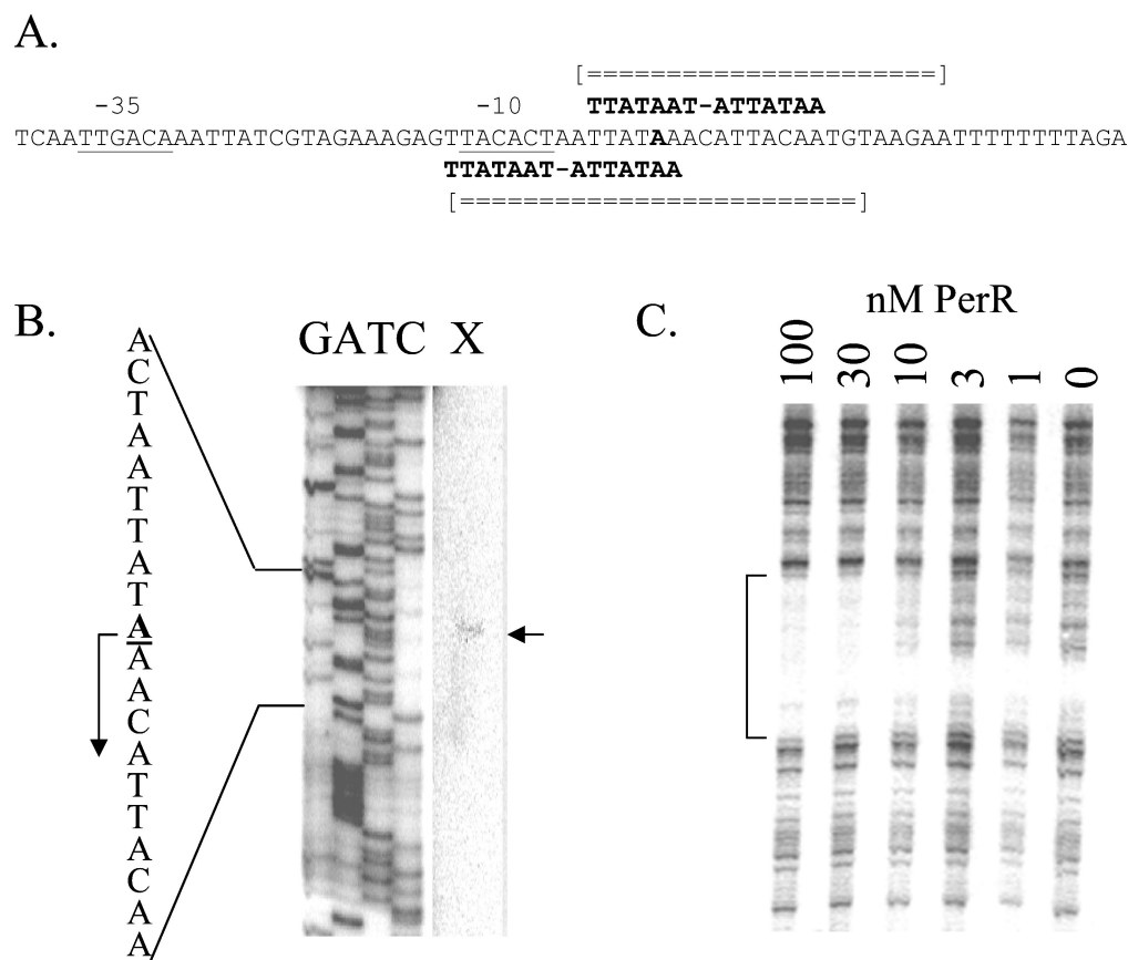
FIG. 1. Interaction of PerR with the perR regulatory region. (A) The -35 and -10 regions of the perR promoter are underlined, and the two overlapping Per box elements are indicated. The A residue start site for transcription is in bold. Regions of both DNA strands protected against DNase I digestion by bound PerR protein are indicated by broken double lines. (B) Primer extension mapping of the perR transcriptional start site (arrow) indicates transcript initiation with the A residue indicated in the sequence to the left. (C) DNase I footprint of purified PerR binding to the perR promoter. PerR was added at the concentrations (nanomolar) indicated in the presence of 10 \mu\text{M} Mn(II). Shown are results from footprinting on the bottom strand; however, top-strand analysis was also performed (data not shown). The regions protected against digestion, as determined by alignment with G+A sequencing ladders (data not shown), are summarized in panel A.
