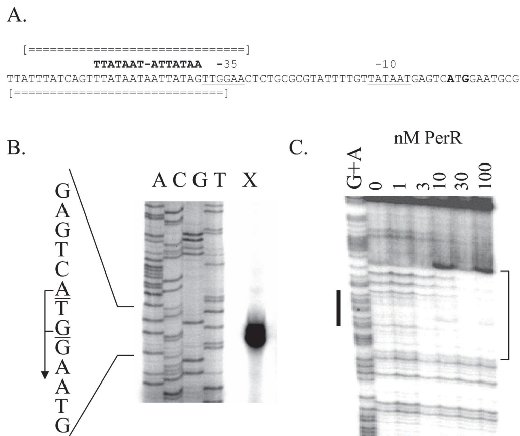
FIG. 2. Interaction of PerR with the fur regulatory region. (A) The -35 and -10 elements of the fur promoter are underlined, and the transcriptional start sites are in bold. The Per box upstream of the -35 element is indicated. Regions of both DNA strands protected against DNase I digestion by bound PerR protein are indicated by broken double lines. (B) Primer extension mapping of the transcription start sites of the fur gene. Transcription initiates at the indicated A and G residues. (C) DNase I footprint of PerR binding to the fur operator region. The results shown are for the bottom strand. Purified PerR was added at the concentrations indicated in the presence of 10\ \mu\text{M} Mn(II). The bold line adjacent to the G+A ladder indicates the position of the Per box, and the protected region is bracketed.
