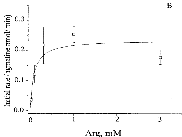
FIG. 6. Concentration dependence of arginine XAR. Wild-type cells were assayed for survival efficiency or the arginine-agsmatine exchange rate. (A) For survival data, the solid curve is calculated with the Hill equation, with a half-maximal concentration of 100 \mu\text{M} and a slope factor of 3.2. (B) Initial transport rate data follow a Michaelis-Menten curve, with a half-maximal concentration of 83 \mu\text{M} . These curves are purely empirical and have no theoretical connotations.
