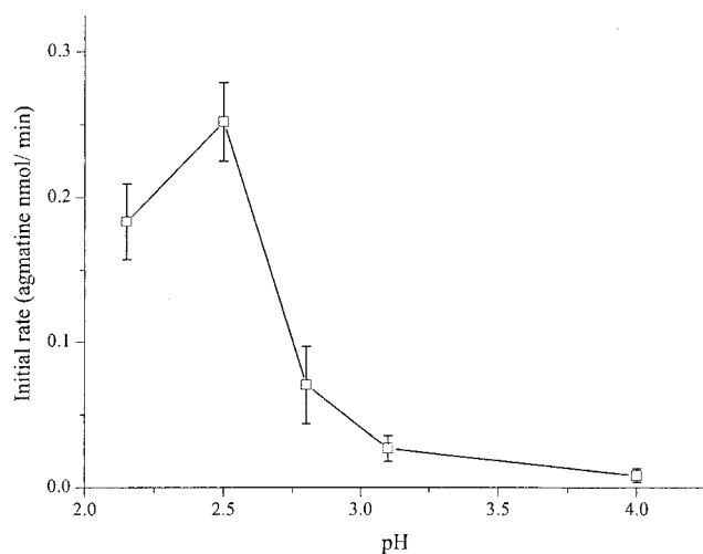
FIG. 5. pH dependence of arginine-agsmatine exchange. The initial rate of agmatine release was measured as a function of pH in the acid shock medium, as described for Fig. 4. Points represent means \pm standard errors of results from triplicate time courses, except for the pH 2.8 data, which show the range of results from duplicate experiments.
