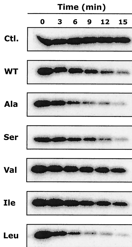
FIG. 6. Dephosphorylation of phospho-PhoP His by the PhoQ-T48X proteins. [ ^{32}P ]phospho-PhoP His was prepared and purified as described in Materials and Methods. Purified [ ^{32}P ]phospho-PhoP His was incubated with either control membranes lacking PhoQ (Ctl.) or membranes containing PhoQ-T48X proteins. At indicated time points, aliquots (15 \mu l) were removed and reactions were stopped by the addition of Laemmli SDS sample buffer. Aliquots were subjected to SDS-PAGE. The amount of ^{32}P associated with the PhoP protein was determined with a PhosphorImager. WT, wild type.
