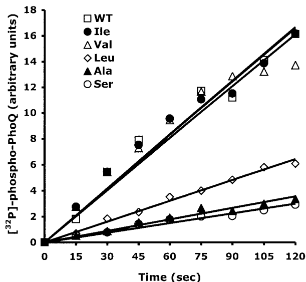
FIG. 5. Initial rates of autophosphorylation of the PhoQ-T48X proteins. Membranes containing wild-type (WT) PhoQ (□), PhoQ-T48A (▲), PhoQ-T48S (○), PhoQ-T48V (△), PhoQ-T48I (●), or PhoQ-T48L (◇) were incubated in the presence of [ \gamma - ^{32} P]ATP and 0.1 mM MgCl_2 for 2 min at 22°C. Reactions (15 \mu l) were stopped by the addition of Laemmli SDS sample buffer. Aliquots were subjected to SDS-PAGE. The amount of ^{32}P associated with the PhoQ protein was quantitated with a PhosphorImager.
