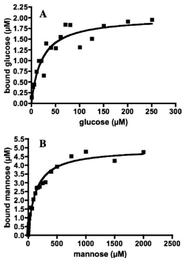
FIG. 3. Binding of glucose and mannose by Mlc_{Tth} . (A) Mlc_{Tth} at 2.5 \mu\text{M} was incubated at 70^\circ\text{C} with ^{14}\text{C} -labeled glucose, and the amount of bound glucose was determined by ammonium sulfate precipitation. The points obtained can be fitted with a Michaelis-Menten curve exhibiting a K_D of 20 \mu\text{M} and binding saturation at 2.1 \mu\text{M} , indicating a stoichiometry of 1:1 (polypeptide-substrate). (B) Mlc_{Tth} at 5 \mu\text{M} was incubated at 70^\circ\text{C} with ^{14}\text{C} -labeled mannose. The points obtained can be fitted with a Michaelis-Menten curve exhibiting a K_D of 134 \mu\text{M} mannose and a binding saturation of 4.76 \mu\text{M} , again indicating a 1:1 stoichiometry.
