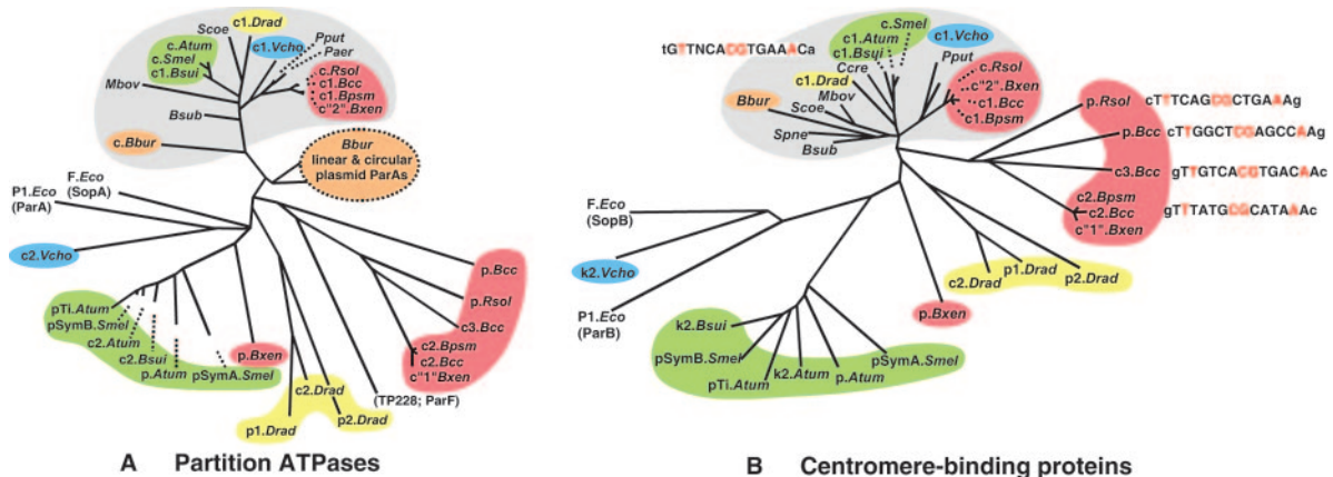
FIG. 3. Phylogeny of partition proteins of bacteria with multipartite genomes. Predicted amino acid sequences of ParA homologues (A) and ParB homologues (B) were aligned and phylogenetically compared using ClustalX. Large blocks of heterology, such as N-terminal extensions present in some ParAs but absent from others, were discarded from the analysis. The option "tree-correct for multiple substitutions" was used. Phylogenetic trees were viewed using Treeview. Homologues of individual multipartite genomes or closely related groups are indicated in color, and others are single-chromosome species included as markers. All branches are of the correct length, but some are extended by dotted lines for clarity. Abbreviations for full species names are as follows: Atum , Agrobacterium tumefaciens ; Bbur , Borrelia burgdorferi ; Bcc , Burkholderia cenocepacia ; Bpsm , Burkholderia pseudomallei ; Bsub , Bacillus subtilis ; Bsui , Brucella suis ; Bxen , Burkholderia xenovorans ; Ccre , Caulobacter crescentus ; Drad , Deinococcus radiodurans ; Eco , Escherichia coli ; Mbov , Mycobacterium bovis ; Paer , Pseudomonas aeruginosa ; Pput , Pseudomonas putida ; Rsol , Ralstonia solenacearum ; Scoe , Streptomyces coelicolor ; Smel , Sinorhizobium meliloti ; Spne , Streptococcus pneumoniae ; Vcho , Vibrio cholerae . The group comprising the largest chromosome of every species, denoted as c or c1, forms a distinct cluster, as shown by the shaded area. Secondary replicons are shown as c2 and c3 or in the case of megaplasmids by their given names or p1 and p2. Large and small replicons of B. xenovorans were named chromosomes 2 and 1, respectively (Joint Genome Institute) and are thus shown in quote marks here. The Borrelia burgdorferi secondary replicon ParBs are less well defined than the ParA group and are not shown. In B, the canonical parS sequence is shown next to the large chromosome group and the parS -like palindromes of B. cenocepacia and R. solanacearum are shown beside their replicons, with conserved bases in red.
