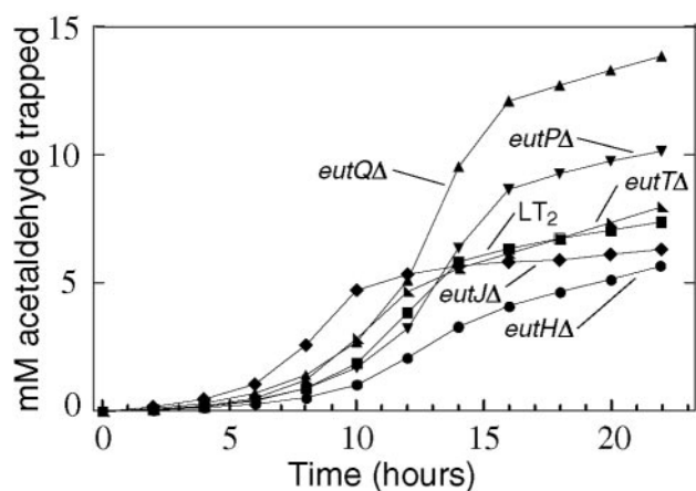
FIG. 6. Effects of other eut mutations on aldehyde release. Mutants eutH (circles), eutJ (diamonds), eutQ (triangles, points up), eutT (right triangles), and eutP (triangles, points down) were compared to wild-type LT2 (squares) for aldehyde release during growth on glycerol, ethanolamine, and B 12 . Ethanolamine was provided at 15 mM.
