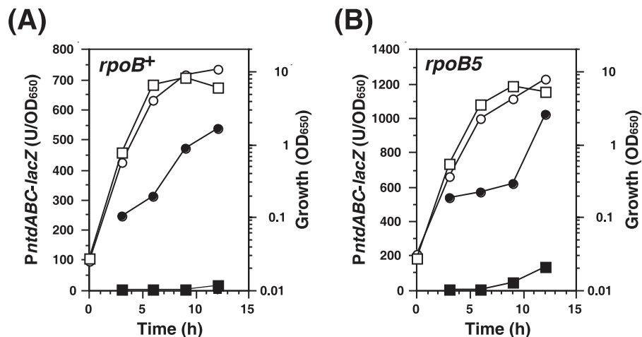
FIG. 3. Effect of glcP mutation on the expression of P_{ntdABC} - lacZ in B. subtilis wild-type and rpoB5 mutant strains. The expression of P_{ntdABC} - lacZ in B. subtilis rpoB+ wild-type (A) and rpoB5 mutant (B) strains is shown. Strains TI122 ( rpoB+ , squares), TI122-UP1 ( rpoB+ glcP ::Tn10, circles), TI122R5 ( rpoB5 , squares), and TI122R5-UP1 ( rpoB5 glcP ::Tn10, circles) were grown in S7N medium containing excess (1%) glucose. Culture samples were withdrawn at the indicated times, and culture densities ( OD_{650} , open symbols) and \beta -Gal activities (closed symbols) were measured. At least three independent experiments were performed, and one of them is shown.
