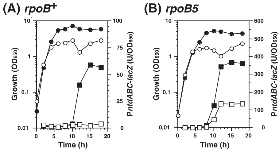
FIG. 2. Growth and transcription of P_{ntdABC} - lacZ in the B. subtilis wild type and rpoB5 mutant strains. Strains TI122 (wild type) (A) and TI122R5 ( rpoB5 mutant) (B) were grown in the presence of limited (0.1%, open symbols) or excess (1%, closed symbols) glucose. Culture samples were withdrawn at the indicated times, and culture densities ( OD_{650} , circles) and \beta -Gal activities (squares) were measured. At least two independent experiments were performed, and one of them is shown.
