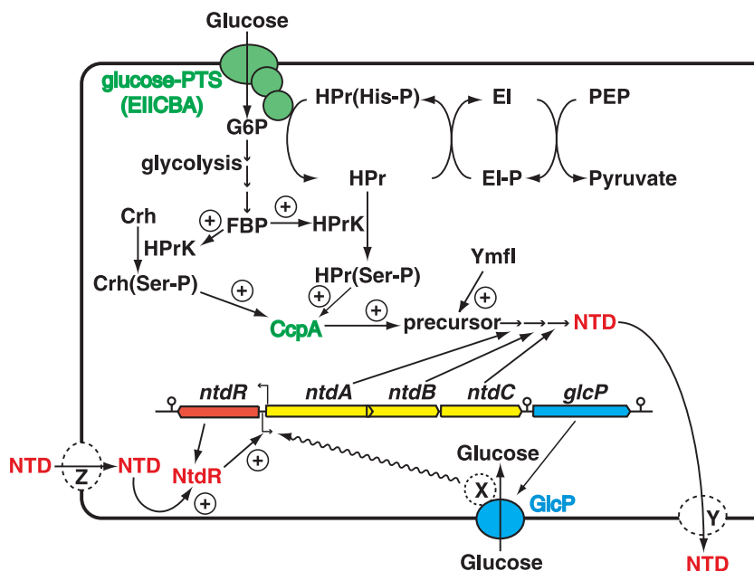
FIG. 8. Proposed model of NTD production in B. subtilis . Glucose transported through glucose-PTS (EIICBA) positively regulates NTD production. This activation mechanism is based on the CcpA-dependent catabolite activation mechanism. Under conditions of high glycolytic activity, fructose-1,6-bisphosphate stimulates the phosphorylation of HPr and Crh at Ser46 by activating HPrK, leading to CcpA-dependent catabolite activation (11). CcpA and YmfI proteins appear to be involved, directly or indirectly, in de novo synthesis of a precursor(s) for NTD, rather than in ntdABC promoter regulation. By contrast, ntdABC is repressed by GlcP-dependent glucose uptake. Possibly, a presumptive transcriptional regulator (designated X) linking to GlcP-dependent glucose uptake participates in this regulation. The transcriptional activator NtdR binds directly to NTD and activates the ntdABC promoter (18). NTD transporters (Y and Z), which are required for export or import of NTD, have not yet been identified. Positive effects are represented as arrows ( \rightarrow ), while the wavy line represents a regulation of the ntdABC promoter by a presumptive transcriptional regulator, X. The glucose-PTS is comprised of enzyme I (EI), enzyme II (EIICBA), and HPr. G6P, glucose-6-phosphate; FBP, fructose-1,6-bisphosphate.
