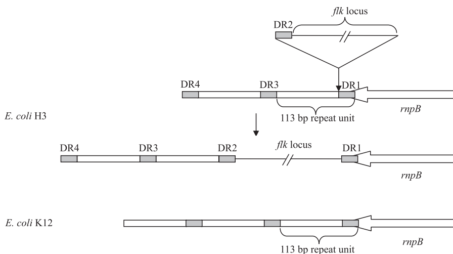
FIG. 2. Schematic representation of the 113-bp repeats downstream of the mpb gene in E. coli strain K-12 and insertion of the flk locus in the same region in the H3 strain. The 113-bp repeats are indicated by open rectangles. The 23-bp sequences corresponding to the last 23 bp of the mpb gene are indicated by shaded rectangles. The positions of DRs in H3 are indicated.
