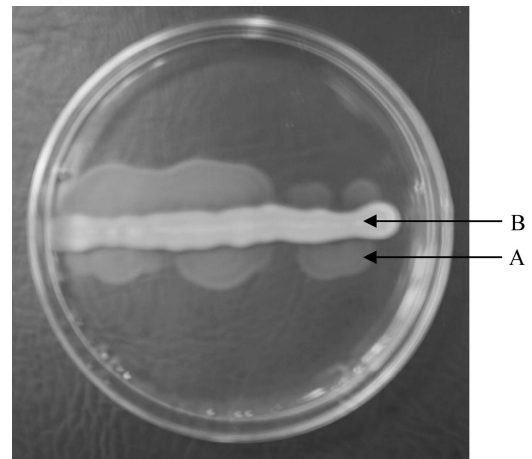
FIG. 5. Selection of spontaneous flagellar phase variants from E. coli H3 on motility agar containing antiserum against H3 antigen. Arrow A indicates spreading growth produced by the phase variants. Arrow B indicates immobilized growth of the H3 parental strain in the presence of H3 antiserum.
